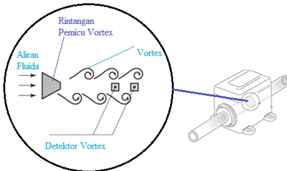
Gambar 0.50 Flow Sensor Vortex
