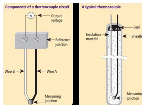
Gambar 0.17 Sensor Termokopel
