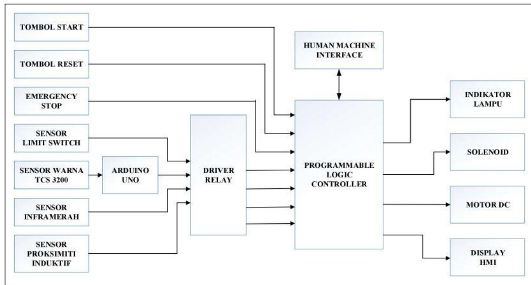
Gambar 6.2. Blok Diagram
