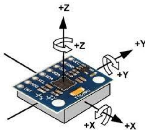
Gambar 0.15 Sensor Girooskop
