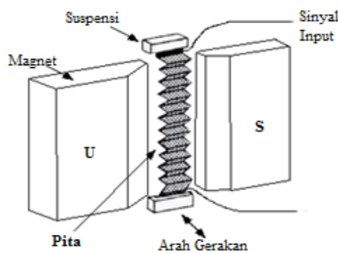
Gambar 0.41 Speaker Pita
