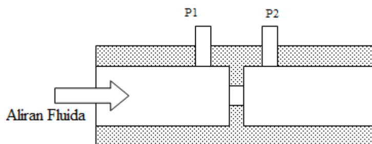
Gambar 0.43 Flow Sensor Orifice Plate
