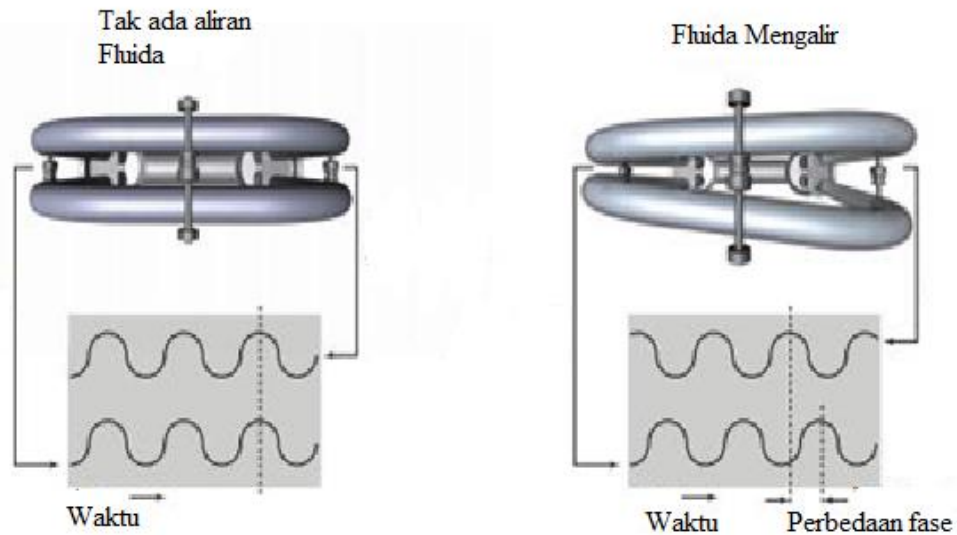
Gambar 0.47 Flow Sensor Coriolis
